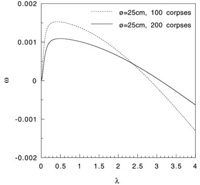
Fig. 4. Stability analysis of the steady states. Solution of the characteristic equation as a function of the wave number \lambda for the experimental conditions \varnothing = 25 \text{ cm} , 100 corpses and 200 corpses. The parameter values are those of Fig. 3 legend.
