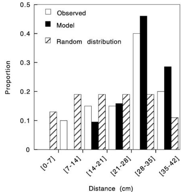
Fig. 6. Comparison between theoretical ( n = 47 ) and experimental ( n = 21 ) distributions of distances between two consecutive clusters in the conditions \phi = 25 cm, 100 corpses and \phi = 25 cm, 200 corpses in the case where only two clusters remain after 24 hr. There is no statistical difference between experimental and theoretical distributions (Kolmogorov–Smirnov test performed on distances, P > 0.334 , Z = 0.945 ) and both distributions are statistically different of a random distribution, n = 5.10^3 (Kolmogorov–Smirnov test performed on distances, P < 0.05 , Z = 1.543 and P < 0.001 , Z = 3.636 respectively). The random distribution is generated as follows: the positions of the two clusters are independent of each other, except that they cannot overlap. The probability that the distance is less than the length of the pile ( L = 4 cm) is 0 and the probability P(l) to have a distance l greater than L and smaller than 0.5\pi\phi is P(l) = 1/[0.5\pi\phi - L] .
